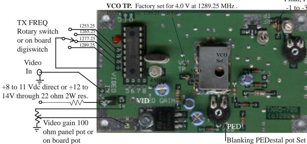
VCO TP. Factory set for 4.0 V at 1289.25 MHz.
