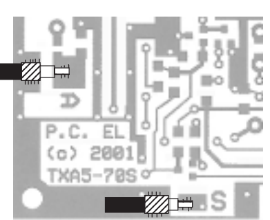
To FMA5 sound board RG174 coax
